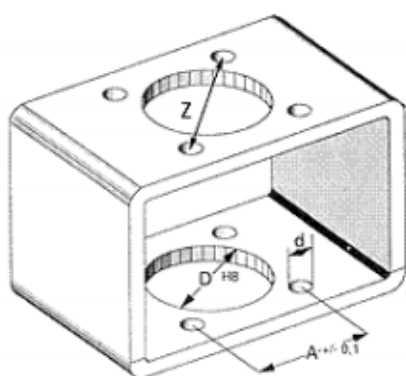
Mounting Bracket
